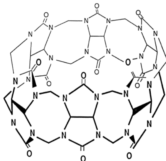
Fig. 1. Chemical structure of cucurbituril.
