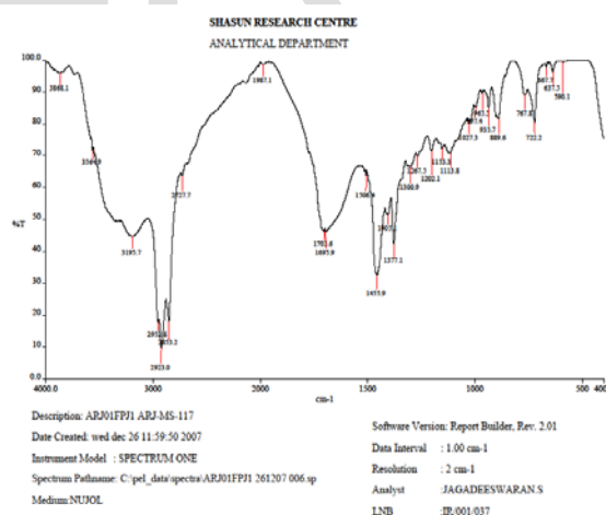
Figure-7 IR-spectra of Cucurbituril
