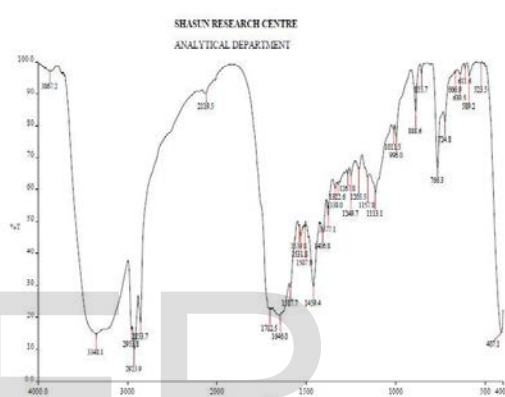
Figure-7 IR-spectra of Cucurbituril
