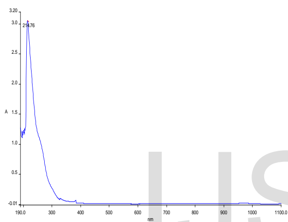
Figure-5 U.V. Absorption spectra of Cucurbituril + Molybdenum II + 2, 2'-Bipyridyl complex with increasing concentration of Cucurbituril (concentrated).
