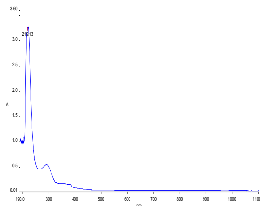
Figure-3 U.V. Absorption spectra of Cucurbituril + Molybdenum I + 2, 2' Bipyridyl complex with increasing concentration of Cucurbituril (concentrated).
